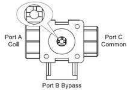
Valve in full flow to coil (C to A)
