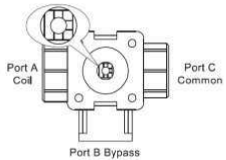
Valve in flow to bypass (C to B)
