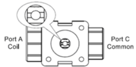
Valve in full flow to coil (C to A)
