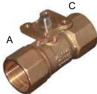
Valve in full flow to coil (C to A)
